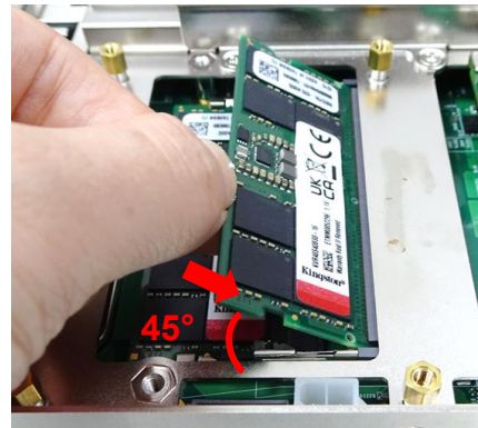
Upper socket
