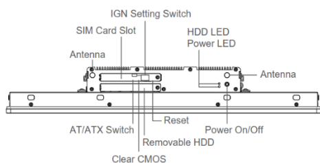
Front I/O
