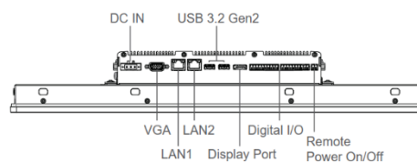
Rear I/O
