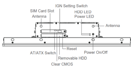
Front I/O
