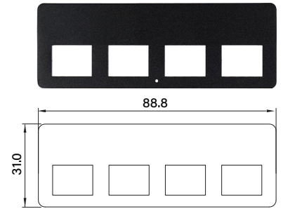
UB1012 Universal Bracket with 4x RJ45 Cutout Dimension (WxD) : 88.8 x 31 mm
