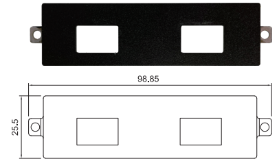
UB1428 Universal Bracket with 2x RJ45 Cutout Dimension (WxD): 98.85 x 25.5 mm
