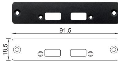
UB1614 Universal Bracket with 2x USB Cutout Dimension (WxD): 91.5 x 18.5 mm
