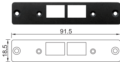
UB1611 Universal Bracket with 2x RJ45 Cutout Dimension (WxD): 91.5 x 18.5 mm
