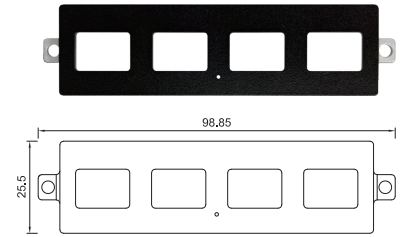
UB1412 Universal Bracket with 4x RJ45 Cutout Dimension (WxD): 98.85 x 25.5 mm
