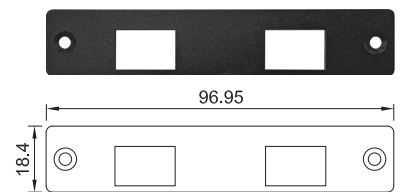
UB1728 Universal Bracket with 2x RJ45 Cutout for CMI-10GLAN Expansion Dimension (WxD): 96.95 x 18.4 mm
