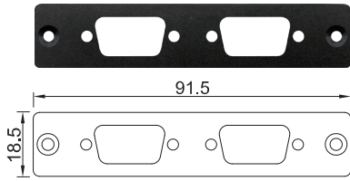
UB1603 Universal Bracket with 2x DB9 Cutout Dimension (WxD): 91.5 x 18.5 mm
