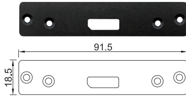
UB1606 Universal Bracket with DP Cutout Dimension (WxD): 91.5 x 18.5 mm
