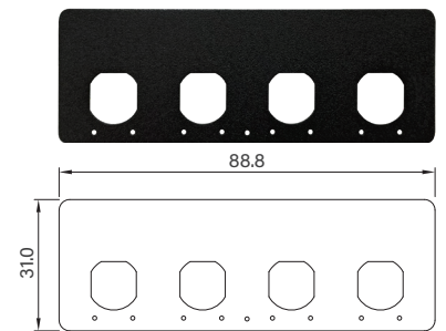
UB1030 Universal Bracket with 4x M12 X-Coded Cutout Dimension (WxD) : 88.8 x 31 mm
