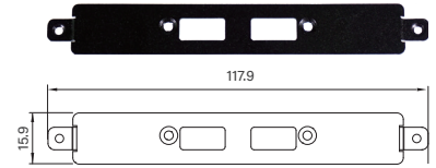
UB1214 Universal Bracket with 2x USB Cutout Dimension (WxD) : 117.9 x 15.9 mm
