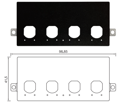
UB1830 Universal Bracket with 4x M12 X-Coded Cutout Dimension (WxD): 98.85 x 41.5 mm
