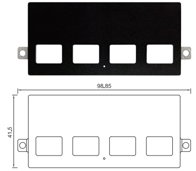
UB1812 Universal Bracket with 4x RJ45 Cutout Dimension (WxD): 98.85 x 41.5 mm
