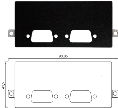
UB1803 Universal Bracket with 2x DB9 Cutout Dimension (WxD): 98.85 x 41.5 mm
