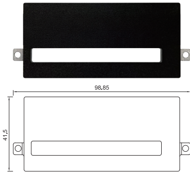
UB1818 Universal Bracket with DIO Cutout Dimension (WxD): 98.85 x 41.5 mm
